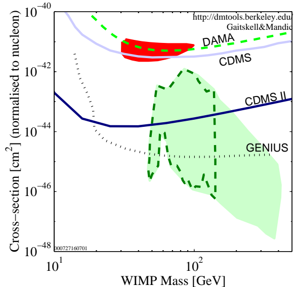
FIG. 2. The cross section for spin-independent \chi -proton scattering is shown. A relatively conservative relic density cut is applied, 0.025 < \Omega h^2 < 1 . Current accelerator bounds, including b \rightarrow s + \gamma are imposed through the DarkSUSY code. The darker region is the DAMA allowed region at 3\sigma CL. The dashed curve is the DAMA 90% CL exclusion limit from 1996 (obtained using pulse-shape analysis). The lighter solid curve is the current CDMS 90% CL exclusion limit, the darker solid curve is the projected exclusion limit for CDMS II experiment and the dotted curve is the projected exclusion limit for the GENIUS experiment. The lighter shaded region is the result of this paper. It represents models allowed within the mSUGRA framework for the constraint m_{1/2} < 1 \text{ TeV} . The closed dashed curve inside this region bounds the region of models allowed in the mSUGRA framework for the constraint m_{1/2} < 350 \text{ GeV} .
