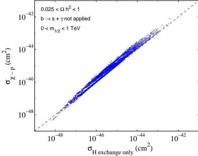
FIG. 3. The cross section for spin-independent \chi -proton scattering: the complete (DarkSUSY) calculation is shown on the y axis and the contribution to the cross section from the Higgs bosons exchange alone is shown on the x axis. A relatively conservative relic density cut is applied, 0.025 < \Omega h^2 < 1 , along with the constraint 0 < m_{1/2} < 1 TeV (instead of 0 < m_{1/2} < 350 GeV).
