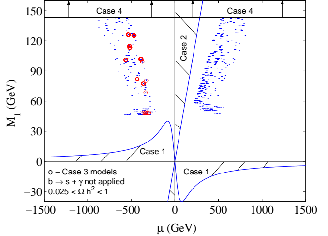
FIG. 4. This figure illustrates the regions of M_1 - \mu plane in which the 4 cases discussed in the text are satisfied. b \rightarrow s + \gamma constraint was not applied, but relatively conservative relic density cut ( 0.025 < \Omega h^2 < 1 ) was applied, along with the constraint 0 < m_{1/2} < 350 GeV.
