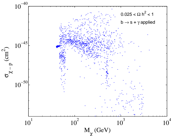
FIG. 6. The cross section for spin-independent \chi -proton scattering in the general MSSM framework is shown. A relatively conservative relic density cut is applied, 0.025 < \Omega h^2 < 1 . Note also that the constraint on the gaugino fraction, z_g > 10 , is applied. Current accelerator bounds, including b \rightarrow s + \gamma are imposed through the DarkSUSY code.
