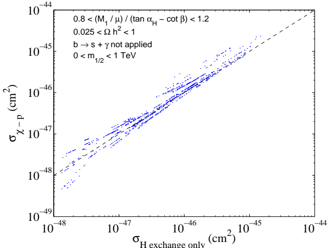
FIG. 5. The proton-neutralino scattering cross section for models where the condition in Case 3 is approximately satisfied. The complete (DarkSUSY) calculation is shown on the y -axis and the contribution to the cross section due only to the exchange of the heavy Higgs boson, H , is shown on the x -axis. A relatively conservative relic density cut is applied, 0.025 < \Omega h^2 < 1 , along with the constraint 0 < m_{1/2} < 1 TeV. The b \rightarrow s + \gamma constraint (along with 0 < m_{1/2} < 350 GeV) eliminates all models shown on this plot.
