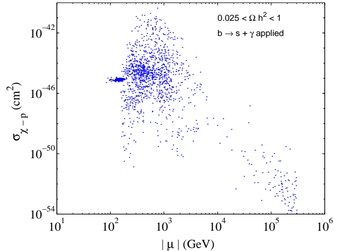
FIG. 7. The cross section for spin-independent \chi -proton scattering in the general MSSM framework is shown. A relatively conservative relic density cut is applied, 0.025 < \Omega h^2 < 1 . Note also that the constraint on the gaugino fraction, z_g > 10 , is applied. Current accelerator bounds, including b \rightarrow s + \gamma are imposed through the DarkSUSY code.
