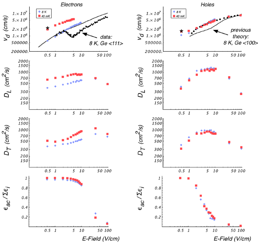
Fig. 1 (Color online) A comparison of electrons and holes, 8 K ( diamonds ) and 40 mK ( squares ). Top graphs show drift velocity compared to pre-existing 8 K theory ( continuous lines ) and experiment ( points ) [1–4]. Asterisks (*) denote data from [8]. The next two rows of graphs show simulated diffusion, longitudinal and transverse. The bottom row shows the ratio of energy dissipated by acoustic phonon emission to that of all phonon emission processes
