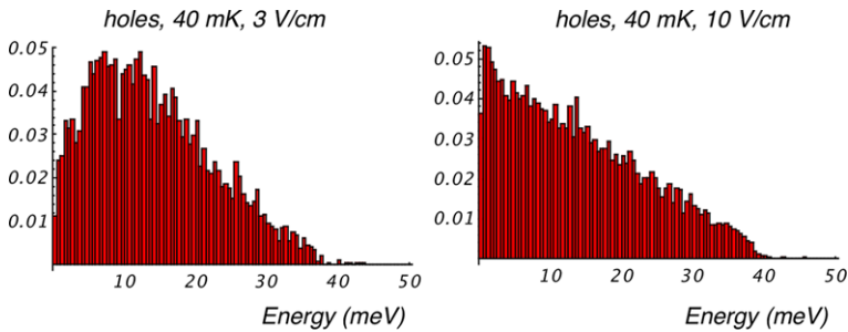
Fig. 2 (Color online) Drift-limited energy distributions at 40 mK. Due to optical phonon emission, carrier energies are not represented well by those of a displaced Maxwellian distribution
