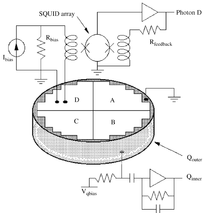
Fig. 1. Schematic of a ZIP detector with its corresponding readout electronics. The four quadrants on the top face are individual phonon sensors. The bottom face is divided into an inner charge electrode separated with a 1 mm gap from an outer guard-ring.
