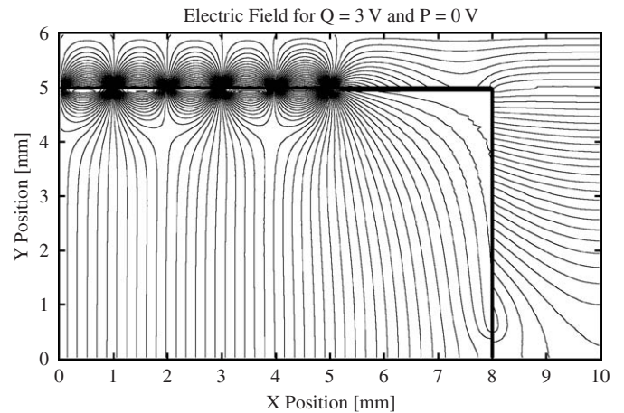
Fig. 3. Calculated electric-field distribution expected for the iZIP electrode configuration with only one quadrant in cross-section shown. Note that the equatorial ground ring maximizes the utility of the surface-ionization scheme to shield the outer perimeter of the detector substrate.
