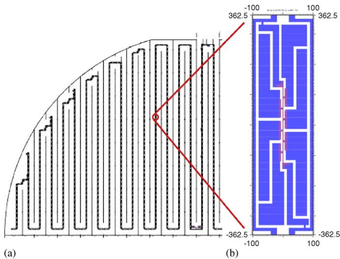
Fig. 2. (a) Design layout for one of the photolithographically patterned phonon sensors on the 76 mm diameter substrate. The phonon sensors are contained within a 200 μm wide ‘ribbon’ that snakes inbetween the interleaving 20 μm wide ionization rails. (b) Zoom-up showing one of the QET [2] elements comprising the phonon sensor. Eight Al athermal phonon collection fins are connected to a 1 μm wide W TES. Superconducting Al rails encompass the QET and supply the voltage bias for all 1246 QETs connected electrically in parallel for each phonon sensor.
