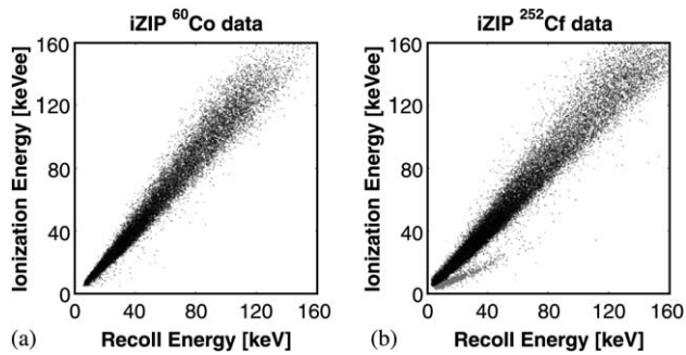
Fig. 5. Preliminary results showing coincident ionization and phonon signals ( |Q_{\text{top}}| + |Q_{\text{bottom}}| vs P_{\text{AD}} + P_{\text{BC}} ) for (a) ^{60}\text{Co} source calibration producing only gamma events, (b) ^{252}\text{Cf} source calibration producing both electron and nuclear recoil events. The nuclear recoil events are clearly identified as the events in the lower band with a relatively reduced ionization yield of \sim 30\% . The energy calibrations shown are only approximate. Some analysis cuts have already been performed on the raw events, as described in the text.
