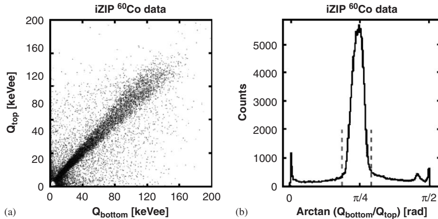
Fig. 4. (a) Ionization signal from the top-surface ( Q_{\text{top}} ) ionization electrode plotted against the bottom-surface electrode ( Q_{\text{bottom}} ) for a ^{60}\text{Co} external source without any analysis cuts. The energy calibration is approximate and given in units of keV electron equivalent. Bulk events within the crystal produce equal (but opposite polarity) charge pulses in both ionization channels, whereas events near one surface (within \sim 700\ \mu\text{m} , see Fig. 3) will only generate events in one of the ionization channels. (b) A histogram in radial angle of (a) showing the response of the ionization channels for the almost uniform irradiation of the 1 cm thick Si substrate. The cut used in subsequent analysis to reject surface events is shown by the (dashed) vertical lines.
