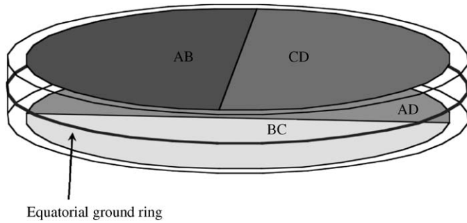
Fig. 1. Schematic of the iZIP (interleaved Z-dependent Ionization and Phonon) detector concept. The metallized equatorial ring defines the ground potential around the perimeter of the detector substrate. The four phonon sensors are arranged to allow the reconstruction of the particle event position in all three spatial coordinates by relative timing and energy collection. The ionization bias electrode ( Q_{\text{top}} ) on the top surface is interleaved with the two phonon channels (labeled AB & CD on the top surface) and the bottom electrode ( Q_{\text{bottom}} ) is interleaved with the two phonon channels (labeled AD & BC) on the bottom surface.
