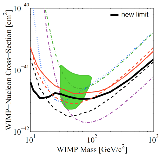
Fig. 2: Spin-independent WIMP-nucleon cross-section vs. WIMP mass. The regions above the curves are excluded at 90% CL. Solid, thick black curve: limit from most recent analysis including statistical subtraction of the neutron background. Solid red curve: limit from this analysis without statistical subtraction of the neutron background. Dashed curves: CDMS expected sensitivity (median simulated limit). Blue dotted curve: previous CDMS upper limit [1]. Above 30 \text{GeV } c^{-2} , the EDELWEISS [6] (purple dot-dashed curve) experiment provides more sensitive limits. Details of the standard Halo model and discussion of DAMA results (green) can be found in Refs. [1,5].
