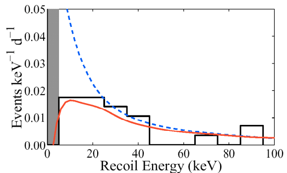
Fig. 1. Histogram of the 20 observed single-scatter nuclear recoil candidates in the 4 Ge ZIPs. The dashed curve is the Monte Carlo simulation predicated shape for the incident neutrons at SUF. The solid curve includes the detector efficiencies and is normalized to the 20 events. All the nuclear recoils observed could be consistent with neutron scattering events. Note that a WIMP with mass below 40 GeV/c 2 is unable, kinematically, to produce events with recoil energy as high as 30-40 keV. Thus the events in this energy range actually observed must be due to neutrons and results in our impressive exclusion limit for low-mass WIMPs.
