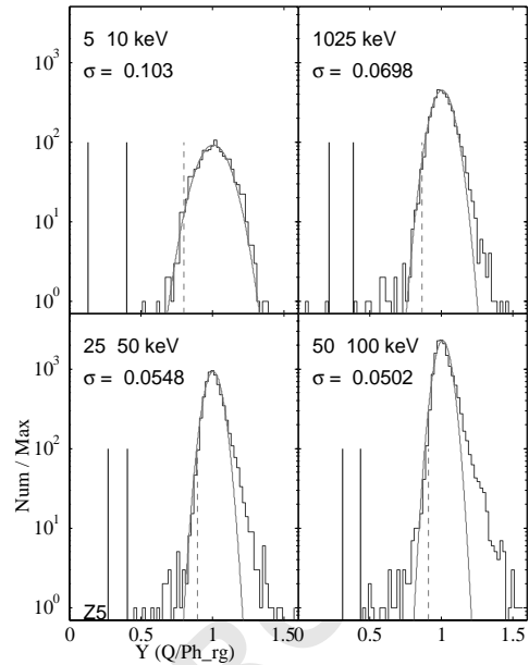
Fig. 1. Histogrammed yield parameter ( Y ) for events in a Ge ZIP detector from an external Co-60 gamma source. The four panes are for the slices in recoil energy ranges considered. Electron-recoil events are calibrated to be centered with a value of Y \approx 1 . The left-hand half of the distribution approximates a simple Gaussian form, as indicated by the fit and \sigma value quoted. The dashed vertical line corresponds to 2\sigma for the Gaussian. The two closely spaced solid vertical lines indicate the 2\sigma acceptance band for nuclear recoils established with neutron source calibrations.
